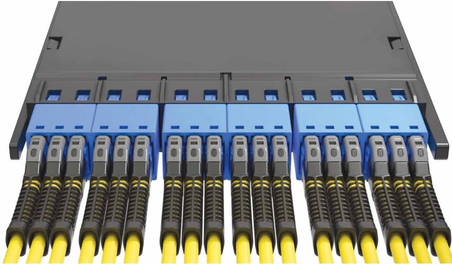
Capacity Increased by 3x Using MDC Connectors and Adapters
