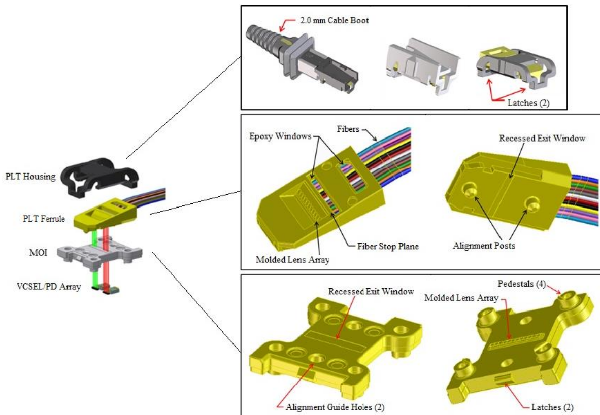
Figure 1. Assembly of the PLT housing, PLT ferrule, MOI, and VCSEL/PD to modularly couple light from the board-level optics to fiber cables. Inset images show a) variations on PLT housings that support both round loose cable fiber and ribbon fiber, b) critical features in the PLT ferrule, and c) critical features on the MOI.
