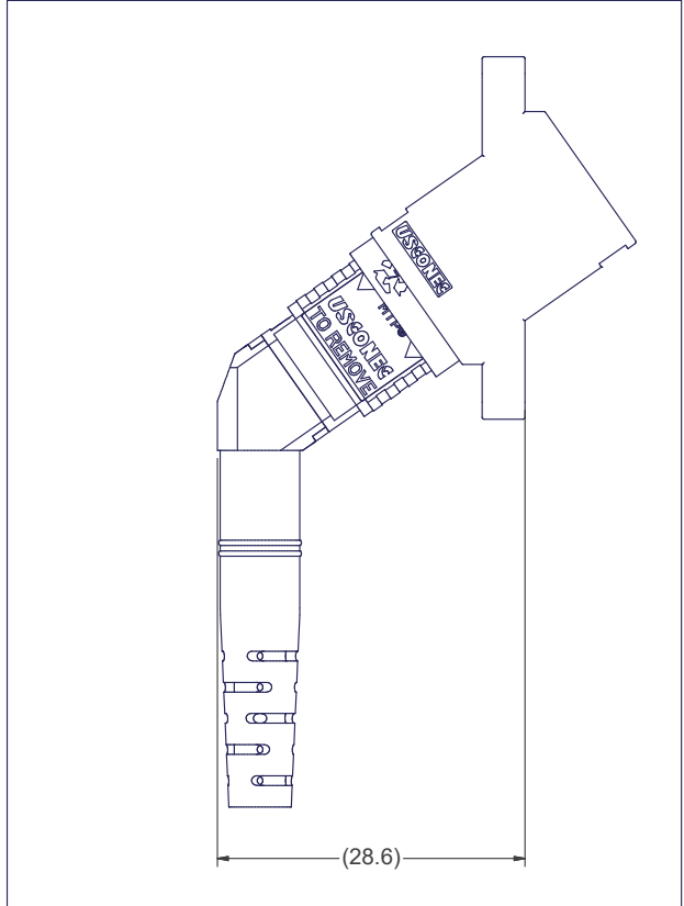
MTP® CONNECTOR SHOWN WITH ANGLED MTP® ADAPTER (ANGLED MTP® ADAPTER SOLD SEPARATELY)
