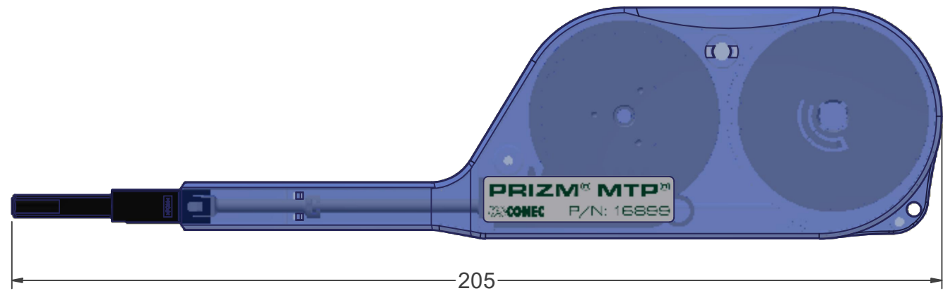
VIEW WITHOUT CAP AND ADAPTER (NOZZLE EXTENDED)
