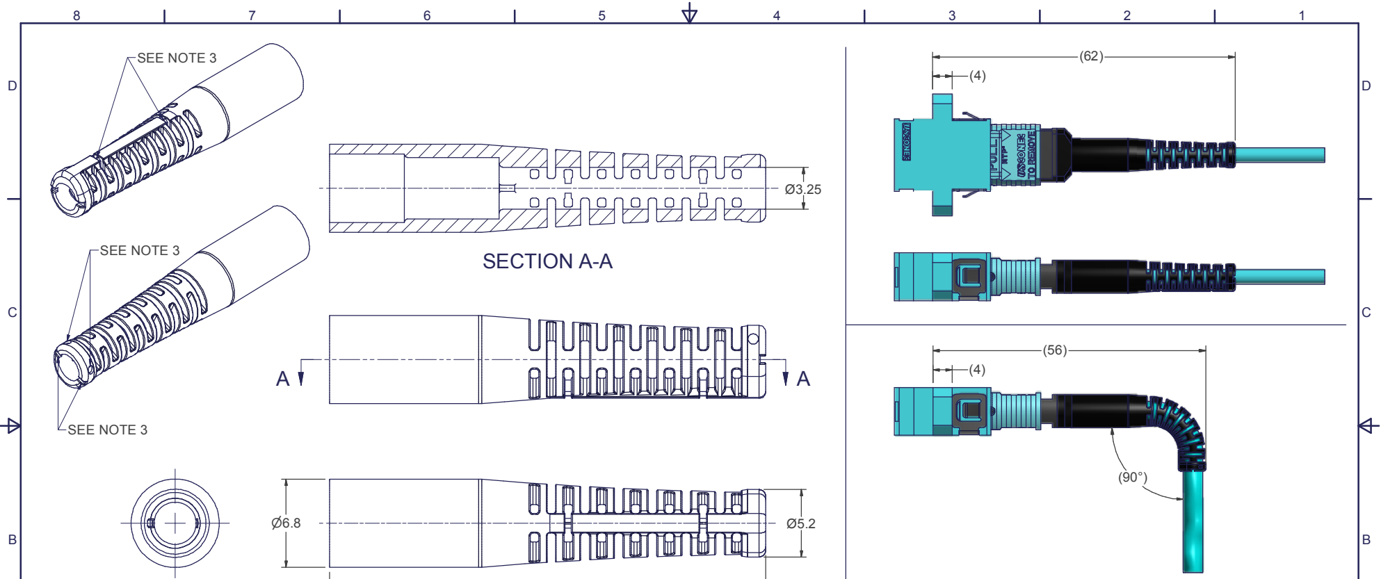
MTP® FLEX BOOT SHOWN WITH MTP® CONNECTOR & MTP® ADAPTER (MTP® CONNECTOR & MTP® ADAPTER SOLD SEPARATELY)
