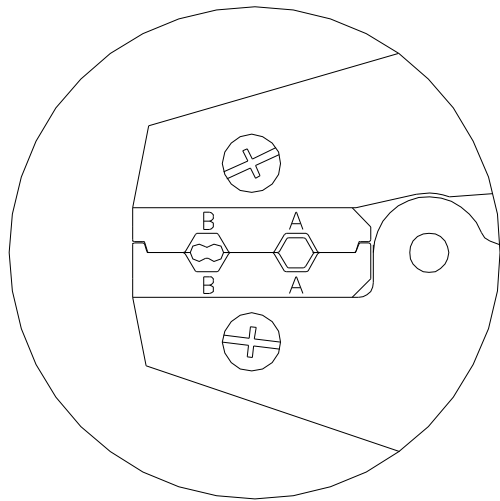
DETAIL 'X'
