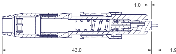
SECTION C-C
